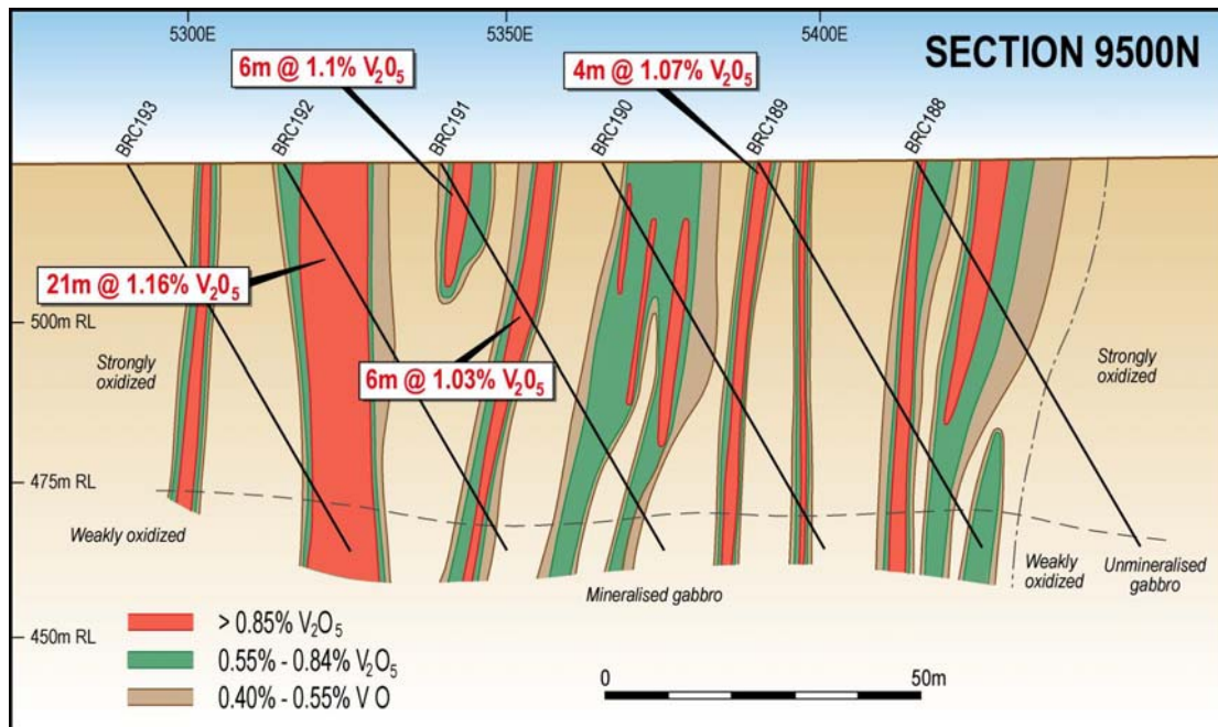
Figure 2 Drill section 9500N at the southern end of the Cove segment of the Barrambie deposit showing interpreted distribution of high-grade (>0.55% V 2 O 5 ) bands (interpretation by Bryan Smith Geosciences). High-grade intersections of the Central Bands (highlighted) are for down-hole intercepts averaging more than 1 % V 2 O 5 , and may include some thin sections of benign dilution (ie, <0.55 % V 2 O 5 ). The drill section is close to the Rabbit Fault, which may have caused some disruption of the massive Eastern Band.
