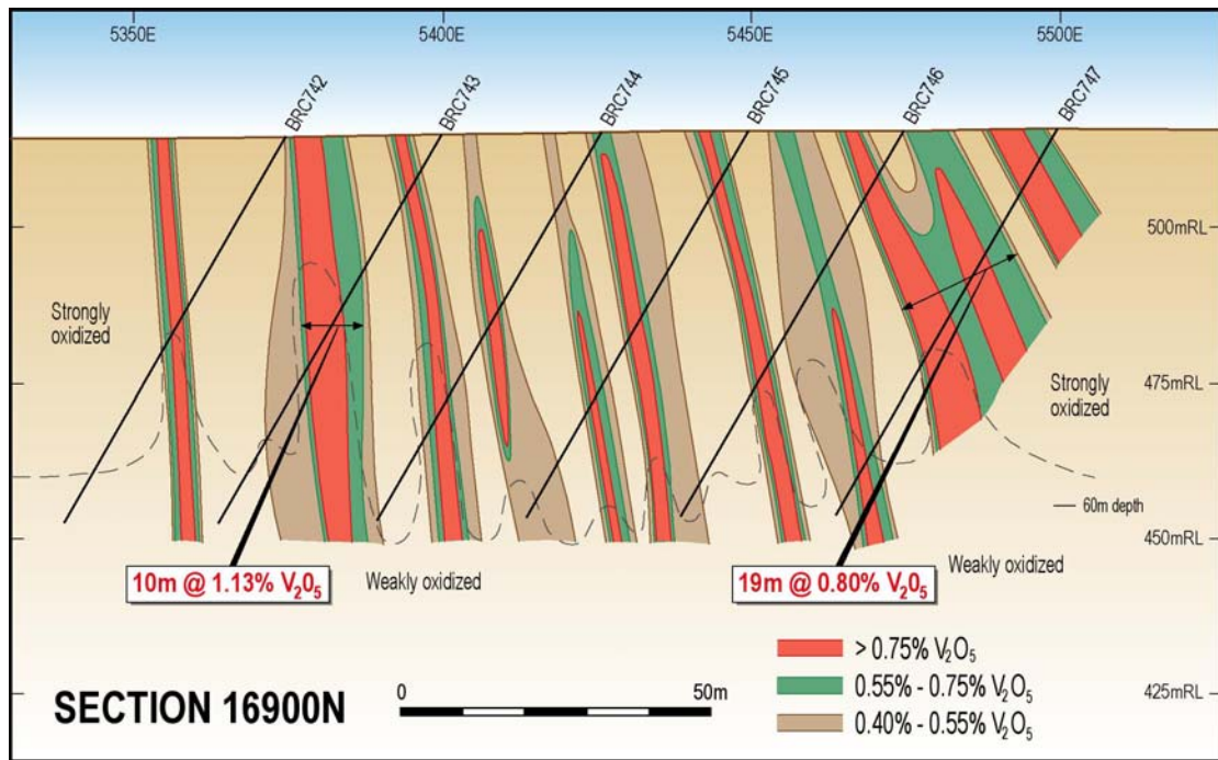
Figure 3 Drill section 16900mN in the central part of the Straight segment of the Barrambie deposit showing the interpreted distribution of high-grade (>0.55% V 2 O 5 ) bands, including several high-grade intersections within the Central Bands (interpretation by Bryan Smith Geosciences). The Eastern Band is the thick band on the eastern (right) side of the section. High-grade intercepts highlighted are for true widths of some of the more significant bands and may include narrow intersections of benign dilution (i.e., <0.55% V 2 O 5 ).
