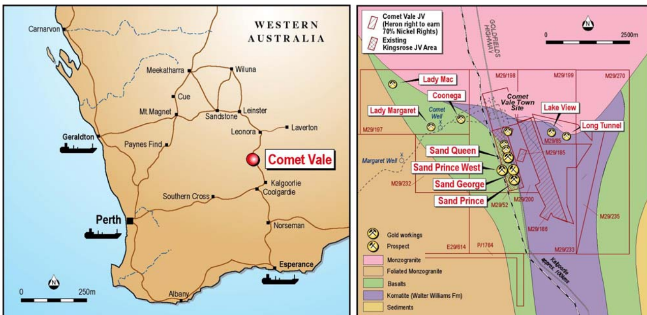
Location of the Comet Vale project (left) and plan of tenements (right) making up the area covered by the revised Joint Venture Agreement.
